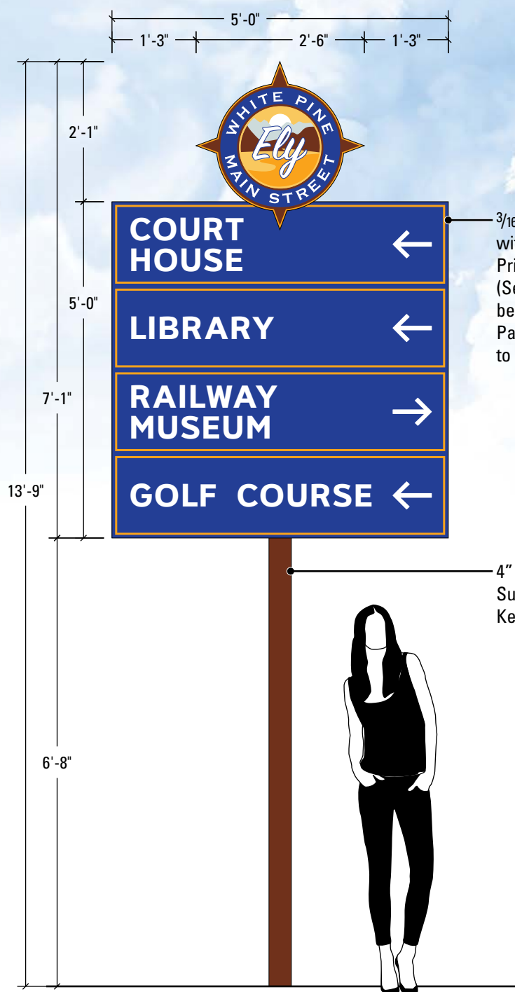
DRAWING 1 SIGN TYPE D1: Directional Sign FRONT VIEW QUANTITY: 2 (See Keystroking) SCALE: 1/2" = 1'-0" KEYSTROKING PENDING
